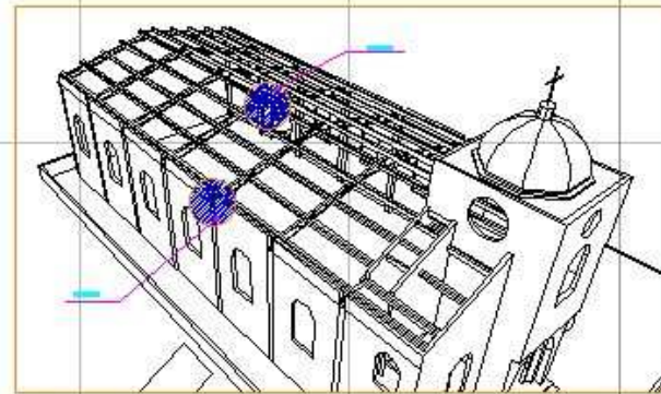
DETAIL 3
